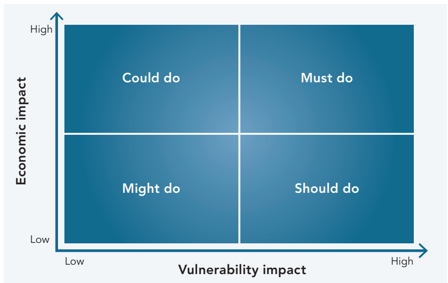
Figure 3: Assessment quadrants
